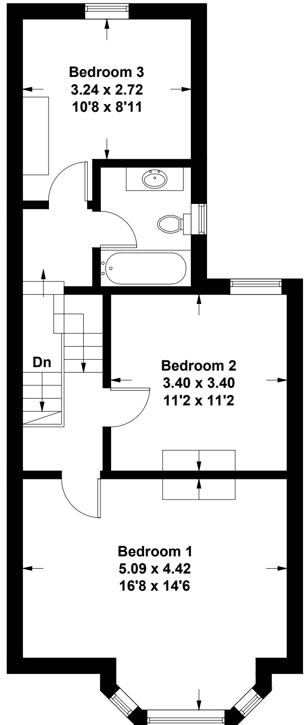
First Floor
