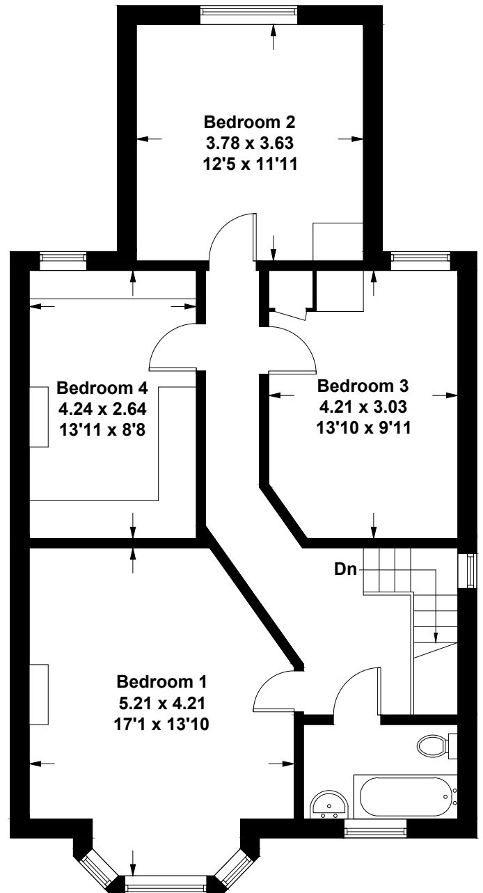
First Floor
