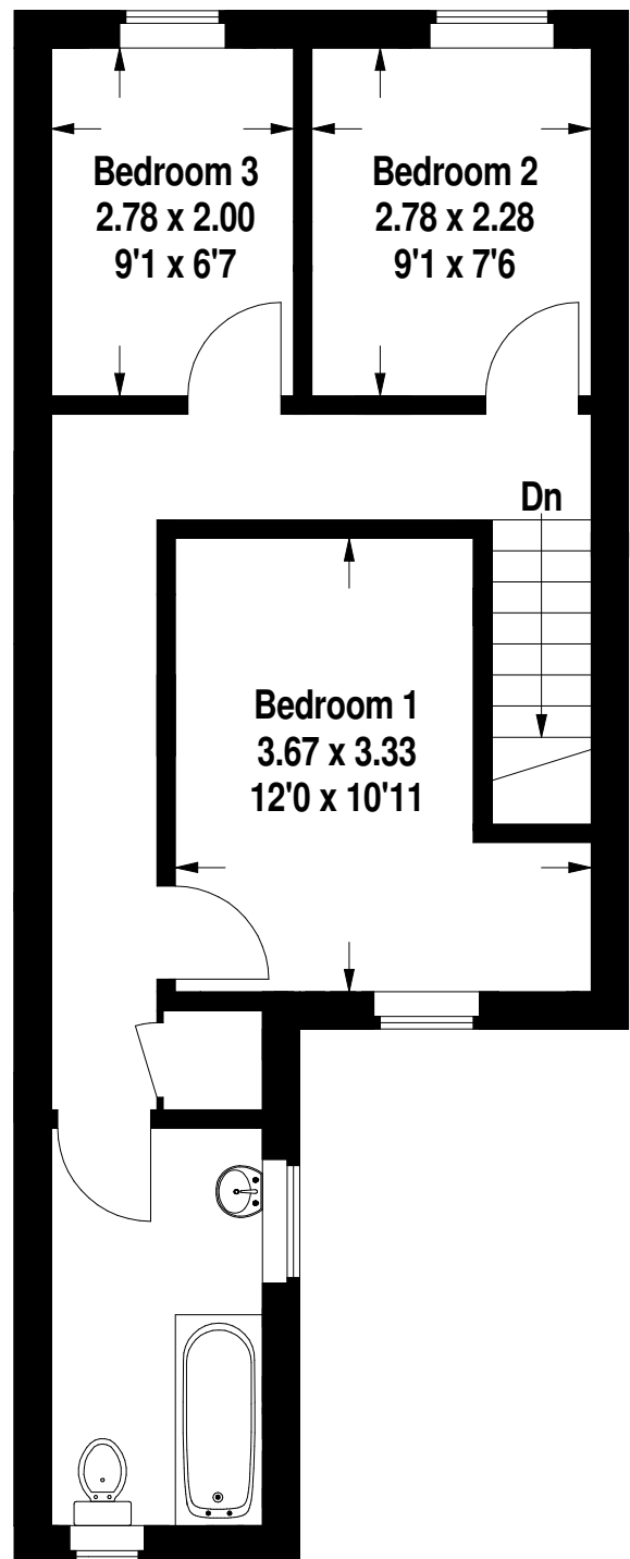
First Floor
